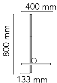
F181110_24W_LED_COORDINATES W2
