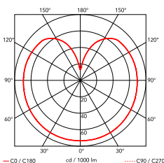
F3010061_13W_LED_GLO-BALL_52
