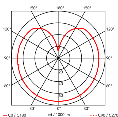
F3026000_13W LED_GLO-BALL C2
