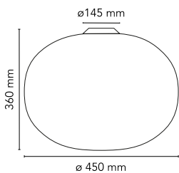
F3026000_13W LED_GLO-BALL C2
