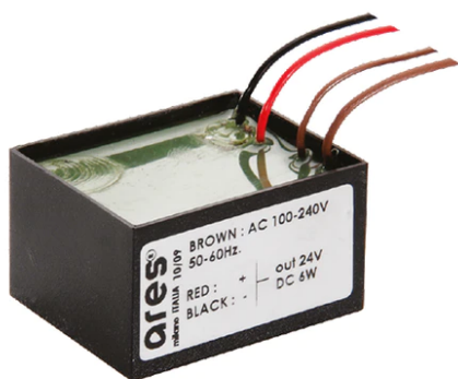
Power Supply 10W 100÷240Vac/ 8W at 24Vdc/ 6W at 350mA Ip65 106
