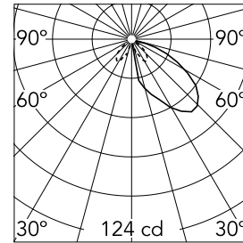
Luminous flux luminaire 295 lm
