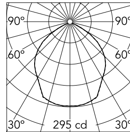
Luminous flux luminaire 657 lm
