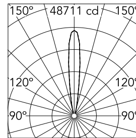
Luminous flux luminaire 3707 lm
