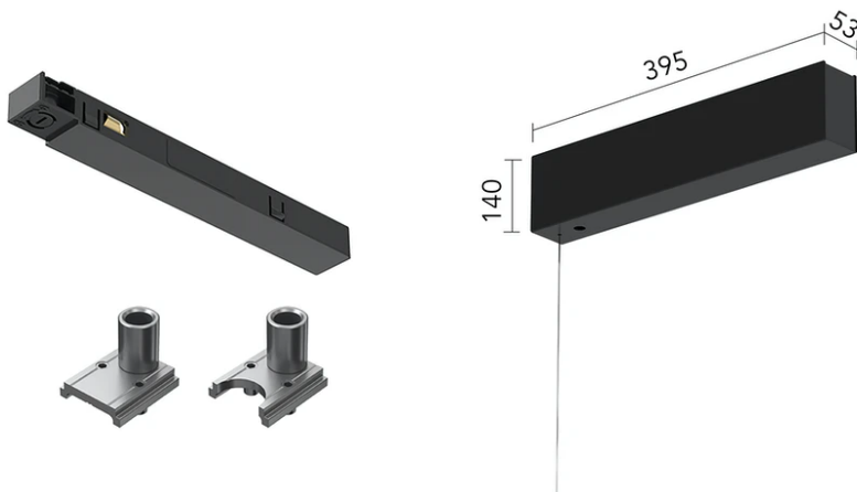
Power connector 08.0626.00
