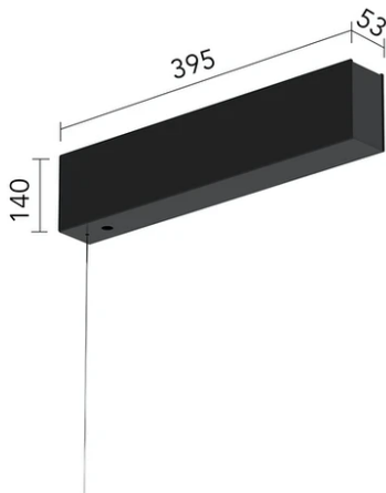
Surface power supply with driver included 320W / 48Vdc. DALI / No dim. 08.0631.14
