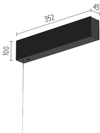
DALI controller and 24V/185W equipment to supply and control both the direct and indirect lighting, included 08.8886.40.DA
