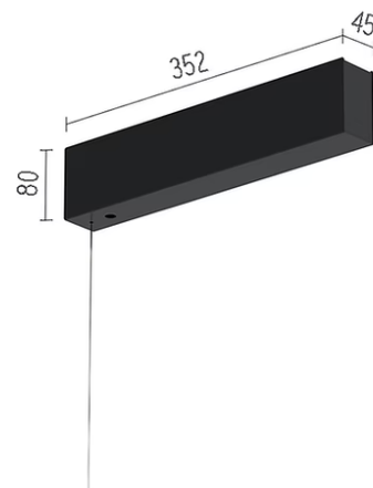
Surface power supply for direct and indirect lighting with housing for the driver 08.8886.40
