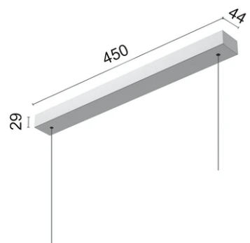
Surface Kit 60W. Dali Version 08.0521.14
