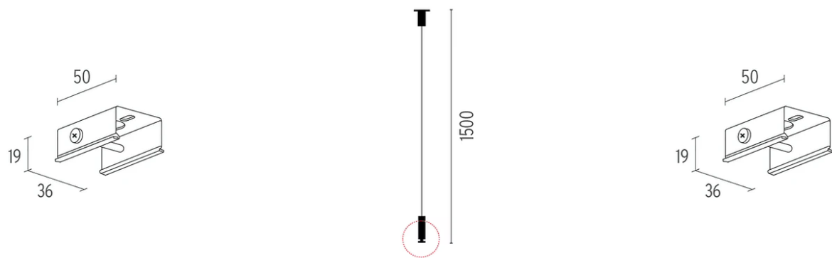
Ceiling fixture or fixture for suspension kit 60.3351.11A
