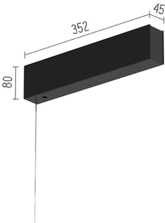
Surface power supply for direct and indirect lighting with housing for the driver 08.8881.14
