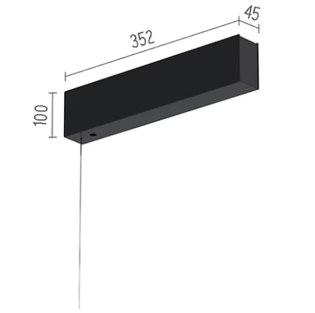
DALI controller and 24V/185W equipment to supply and control both the direct and indirect lighting, included 08.8886.40.DA
