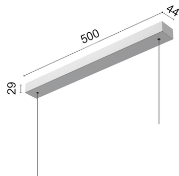
Surface Kit. Non Dimmable/Dali Version 08.0640.40
