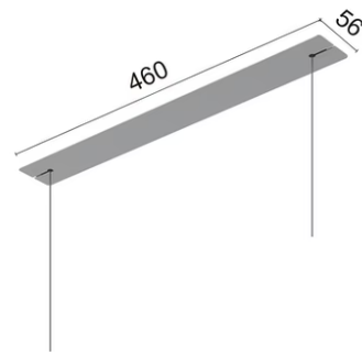
Recessed Kit 60W. Dali Version 08.0523.02
