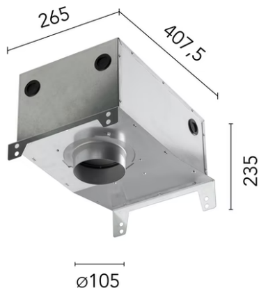
Installation can for concrete 08.8420.00
